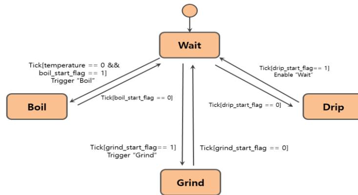
4.2.5.4.2. State Transition Diagram (3.2.1.2)
