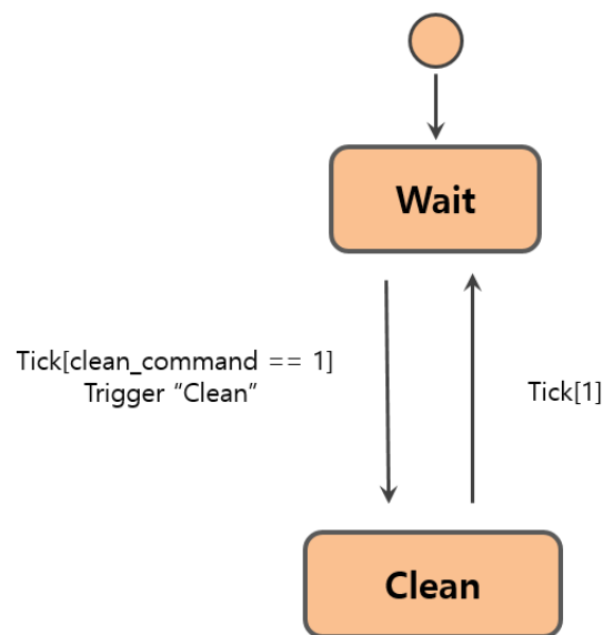
4.2.5.4.2. State Transition Diagram (3.2.1.2)
